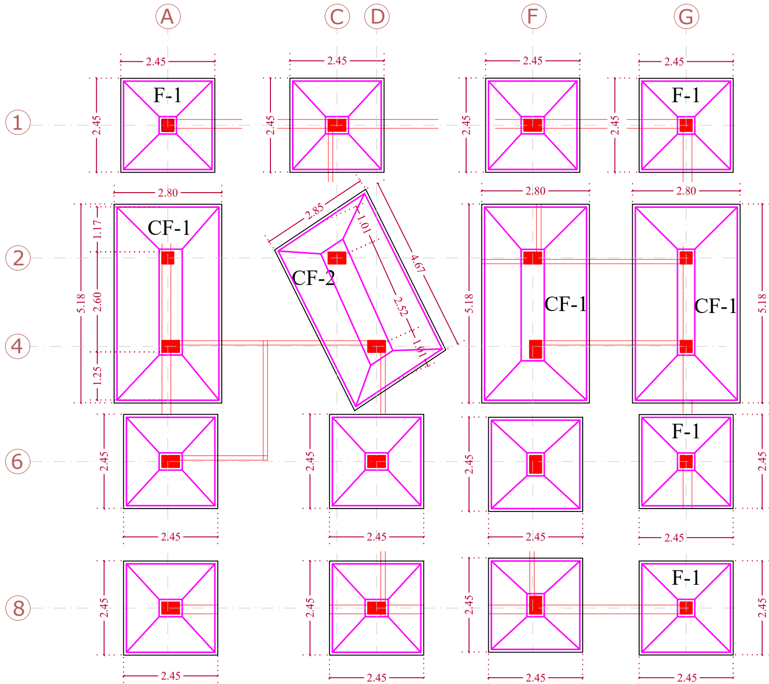
FOOTING LAYOUT
